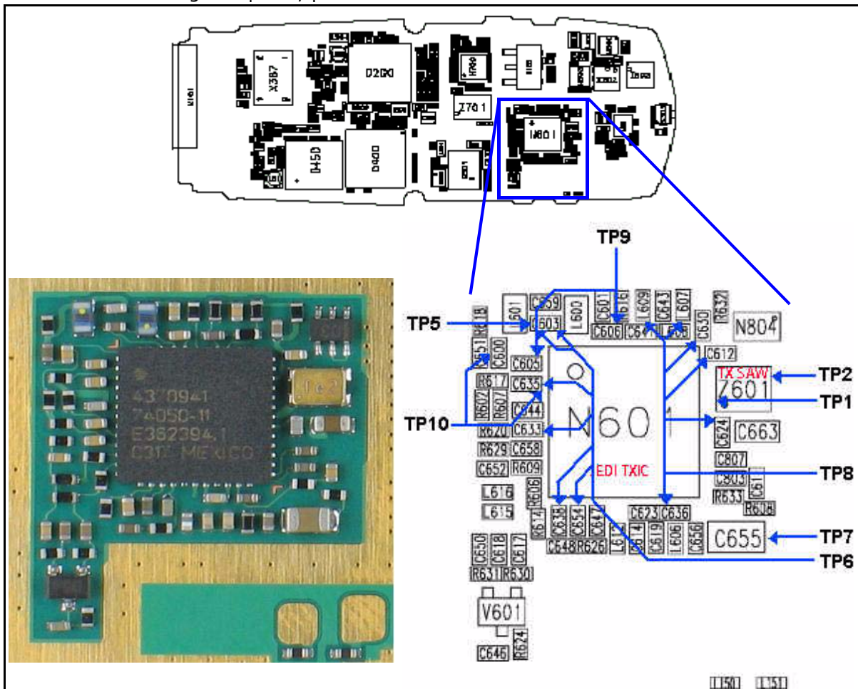
Figure 8: (Top) PWB. (Bottom left) A zoomed view of the testing points on the Jedi TXIC section. (Bottom right) A zoomed view of the Jedi TXIC section with part numbers.
