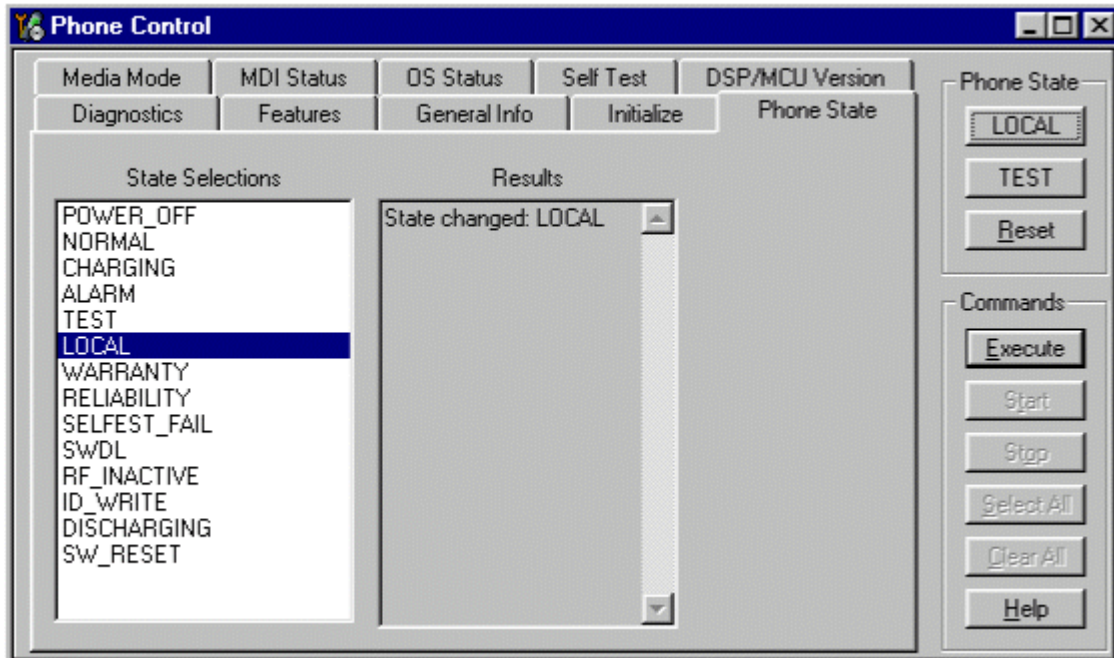
Figure 15: Phone Control dialog box for switching the Rx gain state
