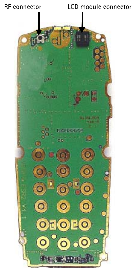
Figure 1: RF components (top)
