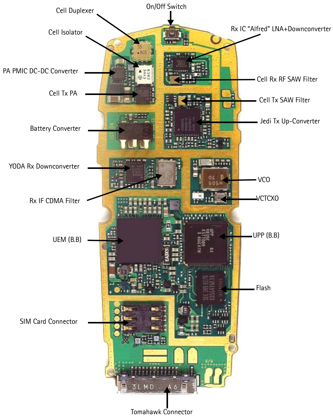
Figure 2: RF components (bottom)
